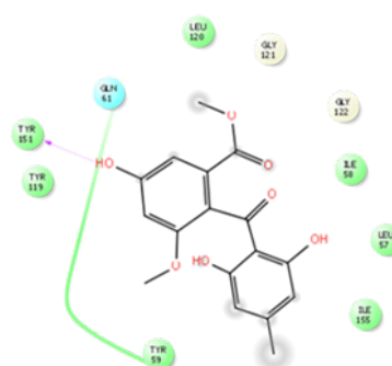
Compound 24 (-4.004 kcal/mol),
