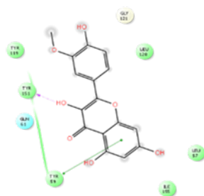
Compound 20 (-4.483 kcal/mol)
