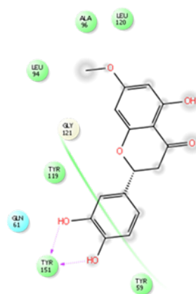
Compound 4: -4.115 kcal/mol
